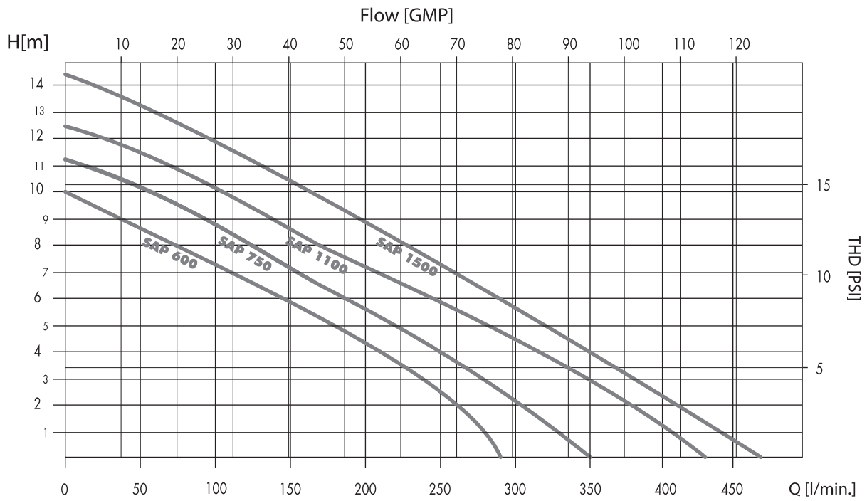
Charakteristika čerpadel SAP Characteristic of SAP pumps
