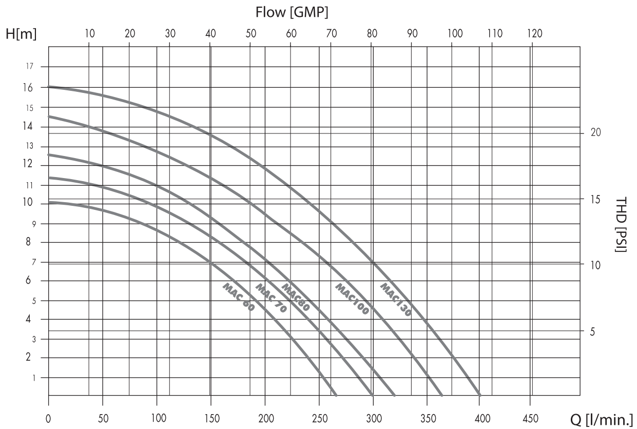
Charakteristika čerpadel MAC Characteristic of MAC pumps
